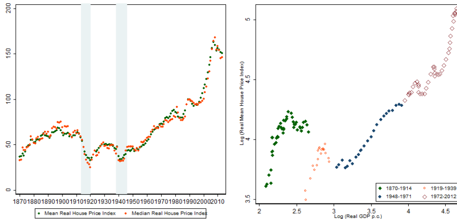
Figure 2: Aggregate Trends.
