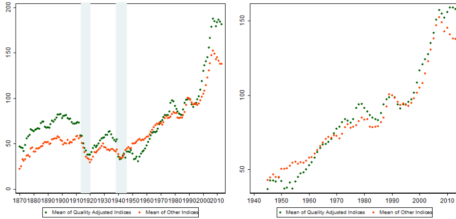
Figure 4: Quality adjustments.
