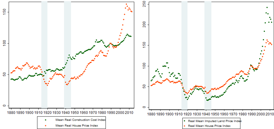
Figure 7: Decomposition.
